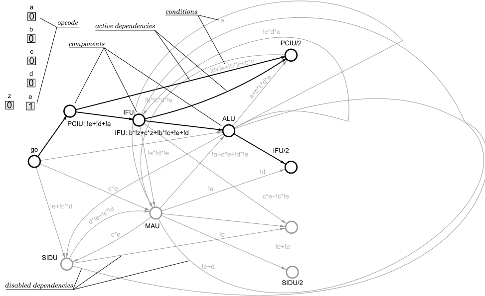
Figure 4: Synthesised CPOG
