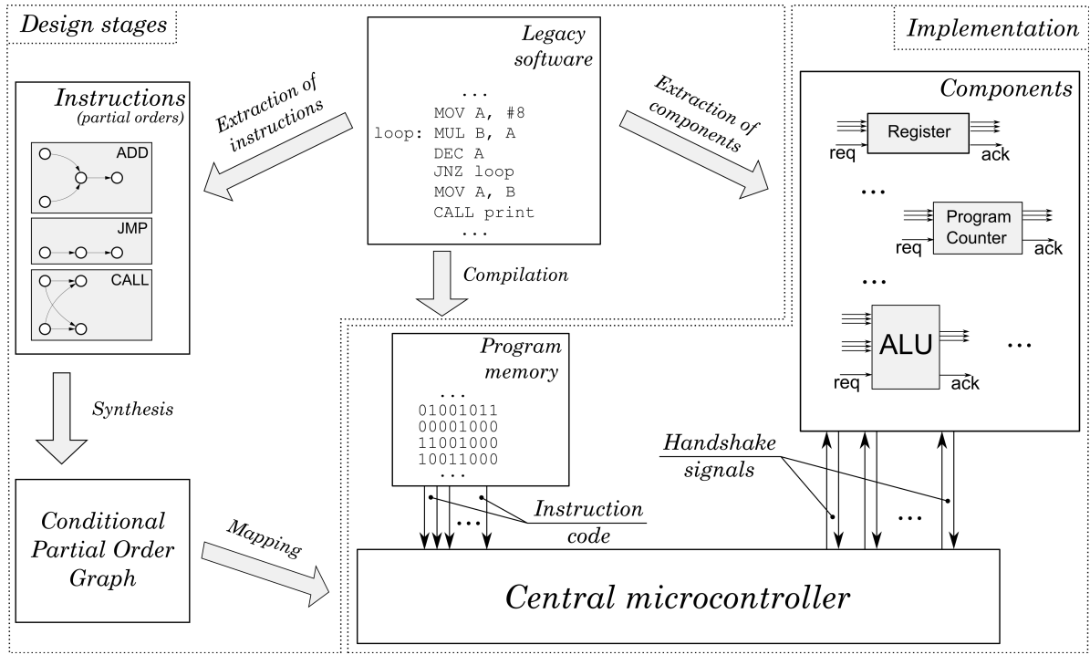
Figure 1: Conceptual view of the design process
