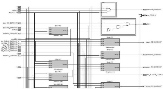
Figure 6: Synthesis of circuit implementation
