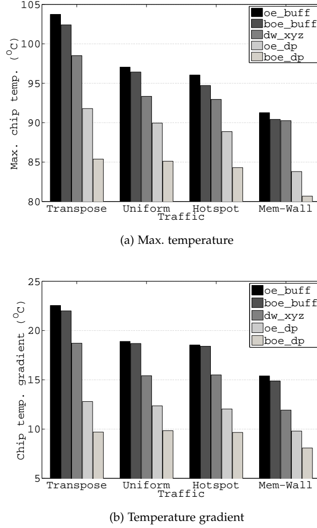
Figure 5.10: Comparison of the maximum and spatial gradient (min.-max.) of chip temperature for the considered routing strategies with various traffic scenarios.
