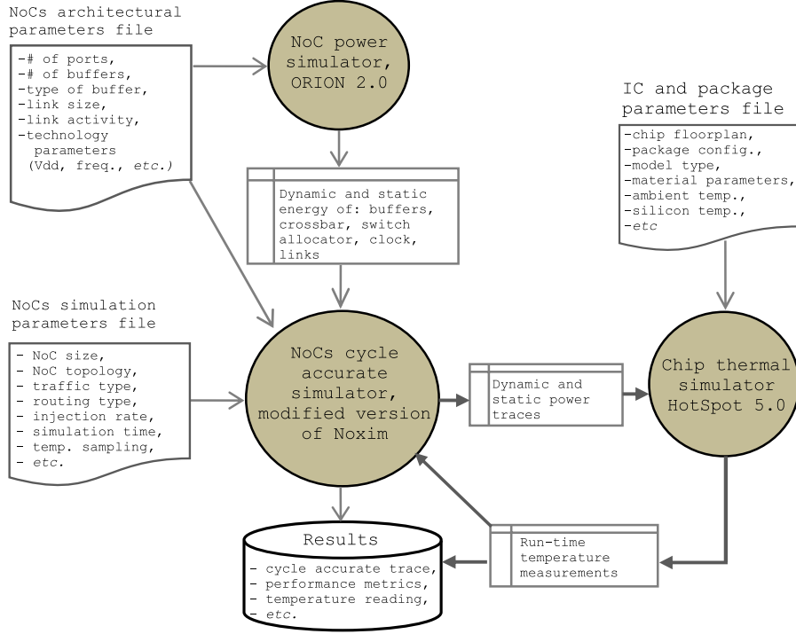
Figure 5.8: Automated computational flow of the proposed tool for dynamic thermal optimization for 3D NoC.
