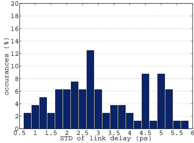
(b) Distribution of links delay (std)
