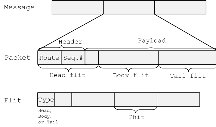
Figure 2.4: Illustration of NoC flow control units of different granularities [109].
