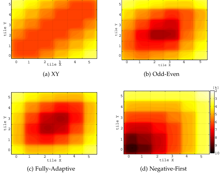
Figure 3.9: Spatial distribution of mean V_{DD} drop (%) for different routing algorithms and Transpose traffic.
