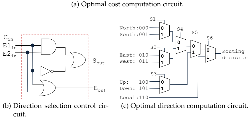
Figure 5.16: Hardware realization of the DP unit.
