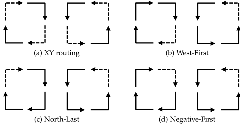
Figure 2.7: Allowable and prohibited turns in XY and turn model routing algorithms in a 2D mesh. Dashed lines indicate prohibited turns and solid lines indicate allowable turns.
